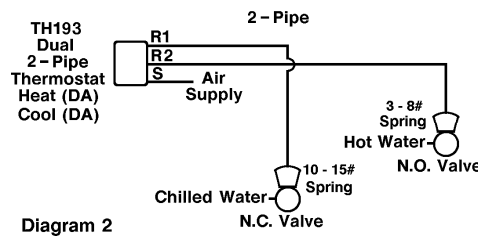
Figure 1. Typical TH 193 HC FEB thermostat Application.
