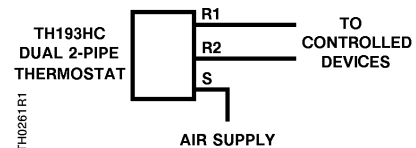
Figure 3. TH 193 HC FEB Thermostat Dual 2-Pipe Connections.
