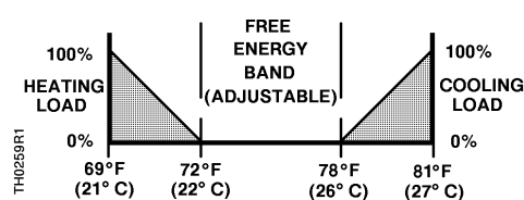
Figure 5. TH 193 HC FEB Operating Characteristics.
