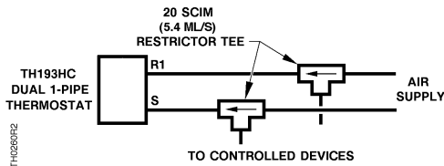
Figure 2. TH 193 HC FEB Thermostat Dual 1-Pipe Connections.
