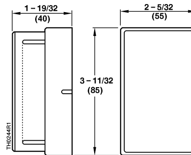
Figure 4. TH 193 HC FEB Dimensions in Inches (Millimeters).
