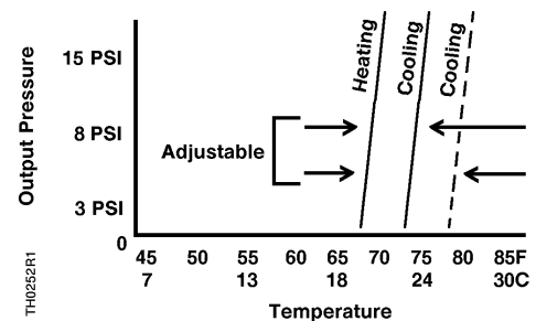
Figure 6. TH 193 HC FEB Input/Output Characteristics.
