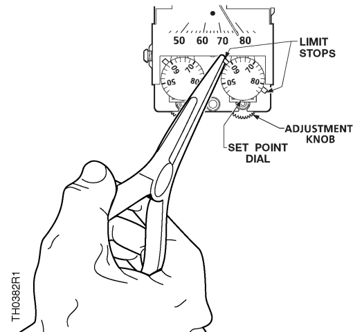
Figure 8. TH 193 HC FEB Limit Stop Adjustments.
