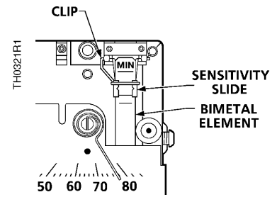
Figure 9. TH 193 HC FEB Sensitivity Adjustment.
